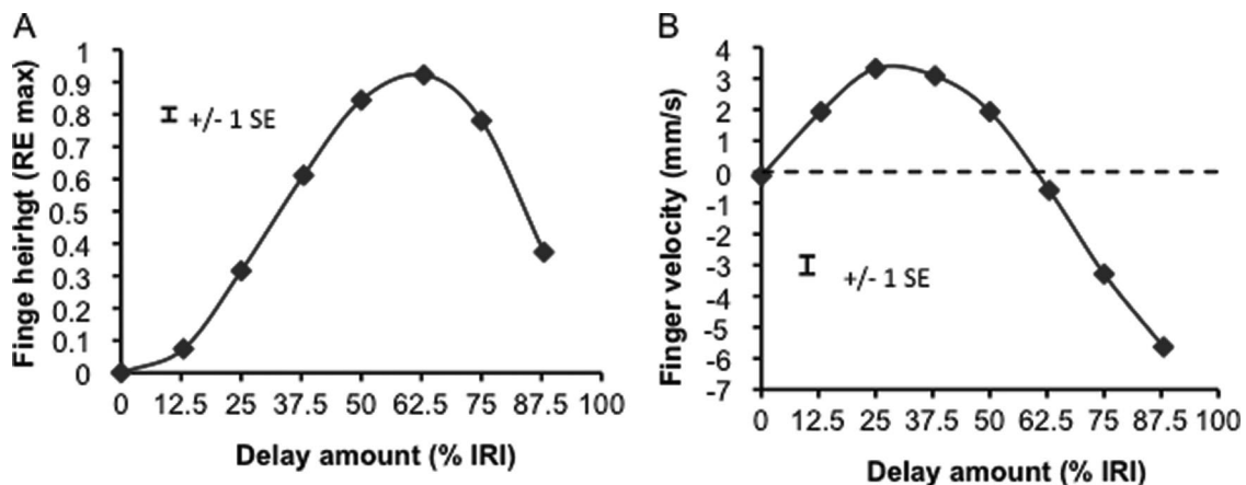
Figure 4. Mean movement state associated with DAF onsets across feedback conditions in Experiment 1: (A) finger position, Z , expressed as proportion of peak within the IRI (Zero indicates surface contact, 1 indicates peak height) and (B) finger velocity ( Z' ). Error bars represent \pm 1 SE.
